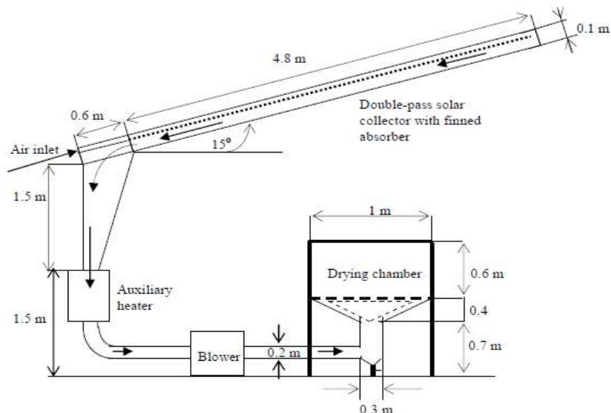
Fig. 9: Schematic diagram of solar assisted drying system
