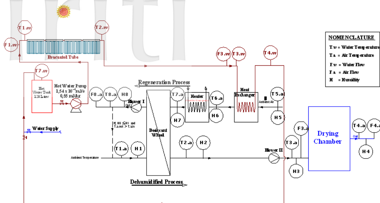
Fig. 26: Schematic diagram of solar desiccant dryer system
