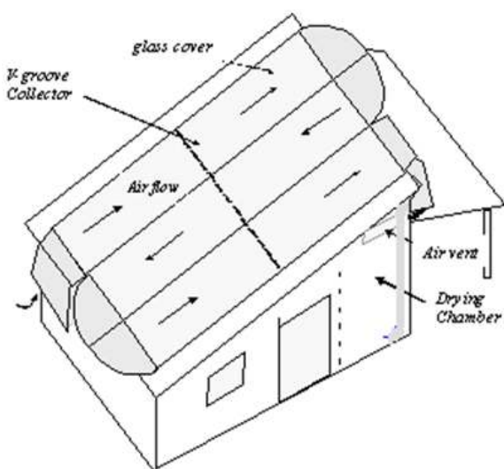
Fig. 14: Configuration of the solar dryer using V-groove absorber
