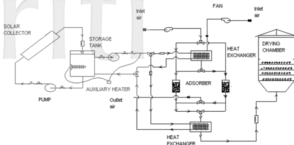
Fig. 24: Schematic diagram of solar assisted dehumidification system
