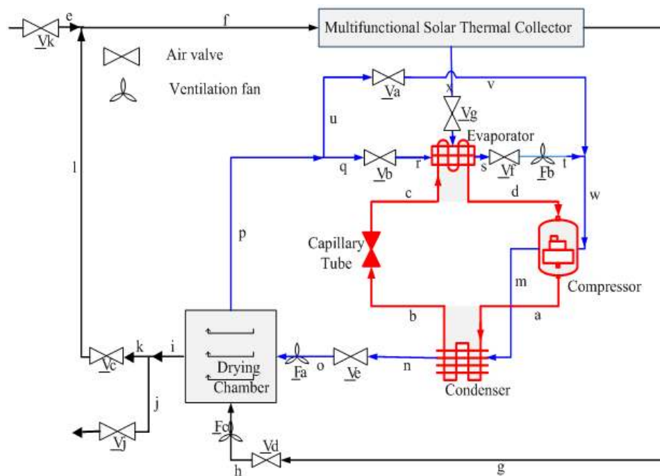
Fig. 18: Schematic diagram of solar assisted heat pump dryer with multifunctional solar collector
