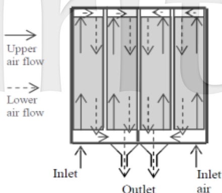
Fig. 10: The collectors arrangement for the solar drying system
