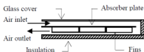
Fig. 11: The schematic double-pass solar collector with fins
