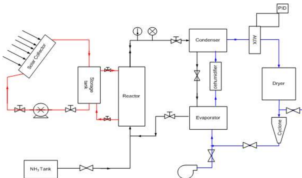
Fig. 23: Schematic diagram of solar assisted chemical heat pump dryer (Ibrahim et al. , 2008)
