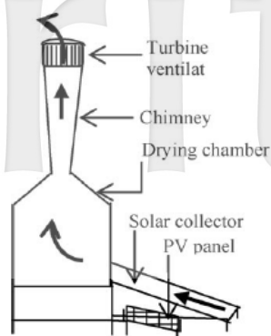
Fig. 3: Schematics of solar dryer system with photovoltaic (PV)
