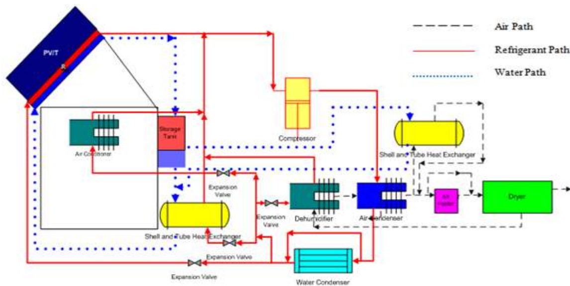
Fig. 20: Schematic diagram of solar assisted heat pump dryer with PV/T water based collector
