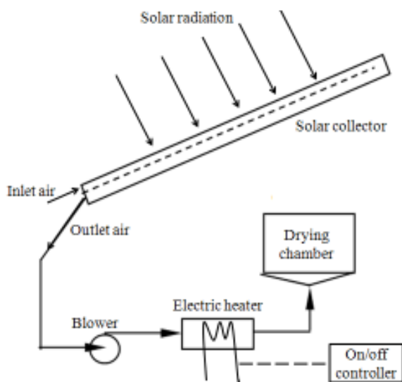
Fig. 6: Schematic of the solar assisted drying system (Sopian et al. , 2007)
