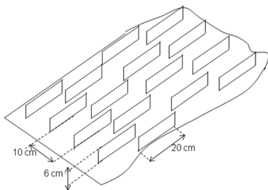
Fig. 12: Top view of the staggered fins absorber
