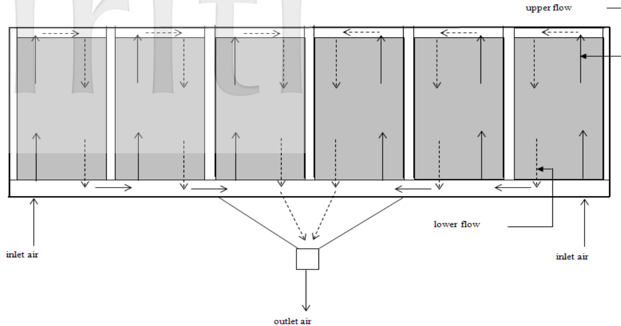
Fig. 7: The collector array for the solar dryer using porous medium (Sopian et al. , 2007)
