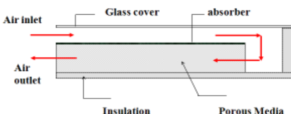
Fig. 5: The double-pass solar collector with porous medium in the second channel (Sopian et al. , 2007)
