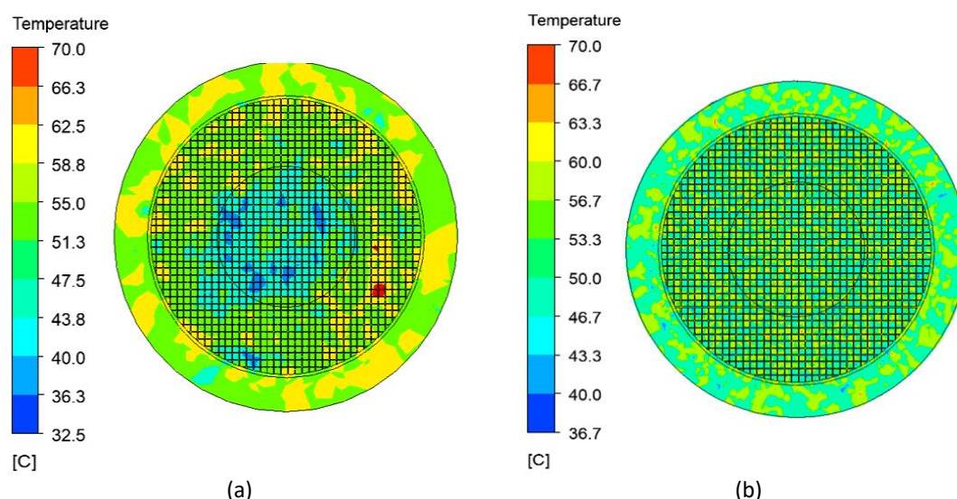
Fig. 8. Contour of temperature in (a) S-SDC and (b) C-SDC
