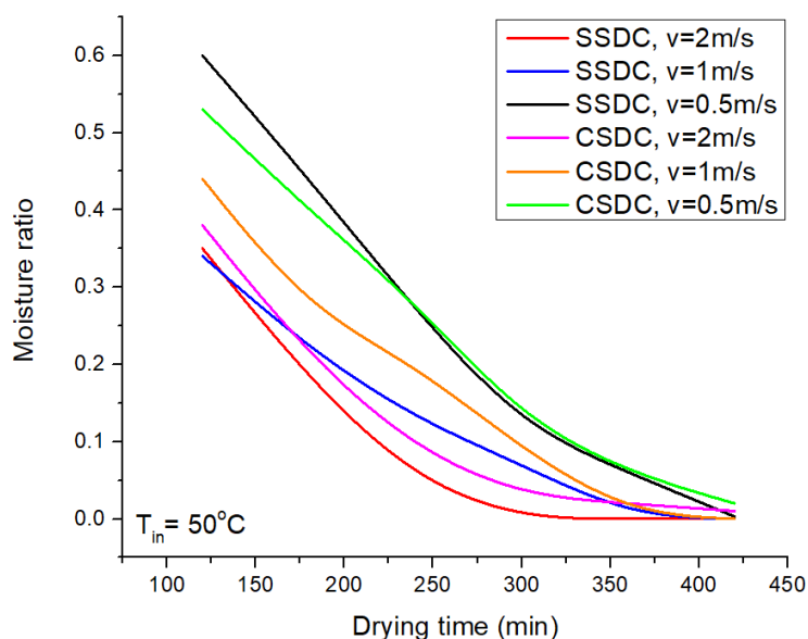
Fig. 11. Relationship between moisture ratio (MR) and drying time (DT, minutes) for kaffir lime leaves at various air velocity in a conventional solar drying chamber (C-SDC) and swirling solar drying chamber (S-SDC) with inclined slotted angle air distributor
