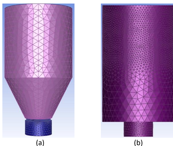
Fig. 4. Generated mesh of solar drying chamber; (a) SSDC, (b) CSDC
