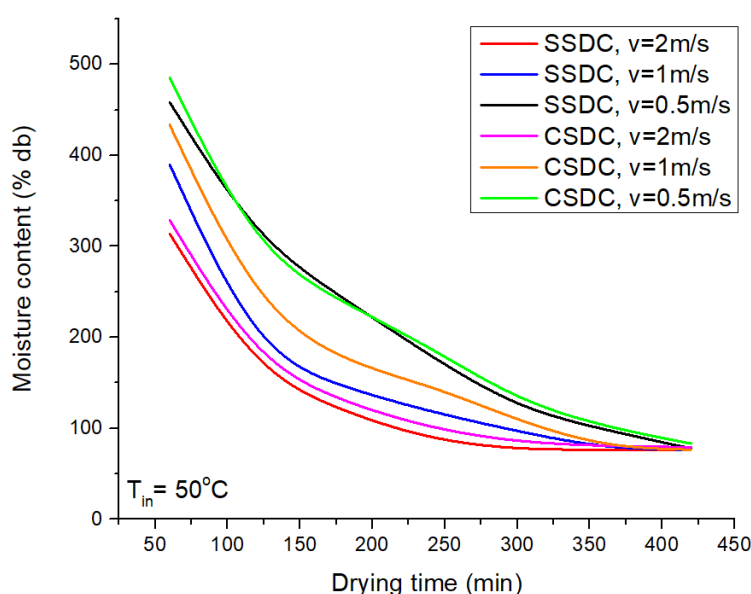
Fig. 10. Relationship between moisture content (MC) and drying time (DT, minutes) for kaffir lime leaves at various air velocity in a conventional solar drying chamber (C-SDC) and swirling solar drying chamber (S-SDC) with inclined slotted angle air distributor
