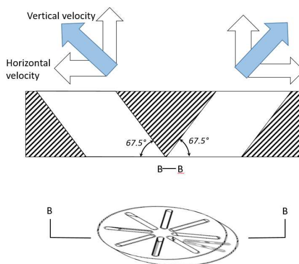
Fig. 2. Details of the inclined slotted angle air distributor
