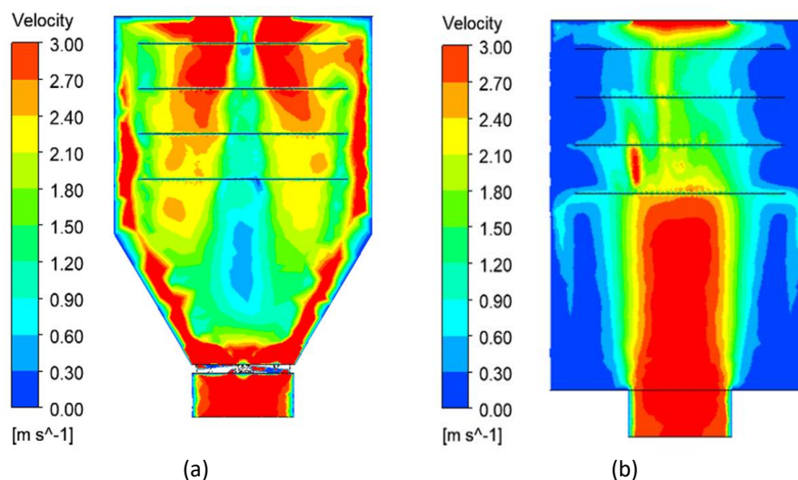
Fig. 7. Contour of velocity contours results for (a) S-SDC and (b) C-SDC
