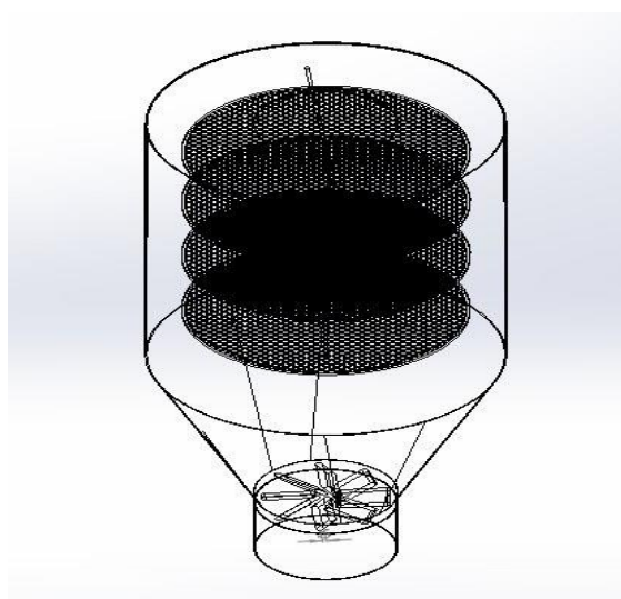
Fig. 1. Details of the swirling solar drying chamber with inclined slotted angle air distributor installed at the bottom of the chamber
