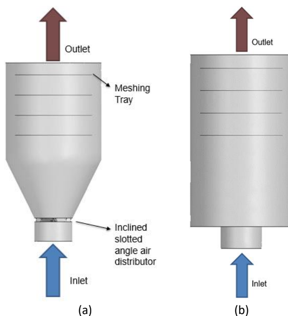
Fig. 3. Boundary condition of solar drying chamber; (a) SSDC, (b) CSDC
