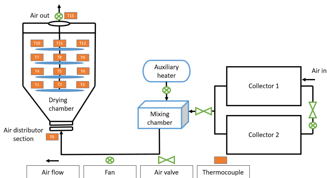
Fig. 5. Schematic diagram of the solar drying system with thermocouple location
