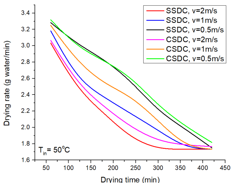
Fig. 12. Relationship between drying rate (DR) and drying time (DT, minutes) for kaffir lime leaves at various air velocity in a conventional solar drying chamber (C-SDC) and swirling solar drying chamber (S-SDC) with inclined slotted angle air distributor
