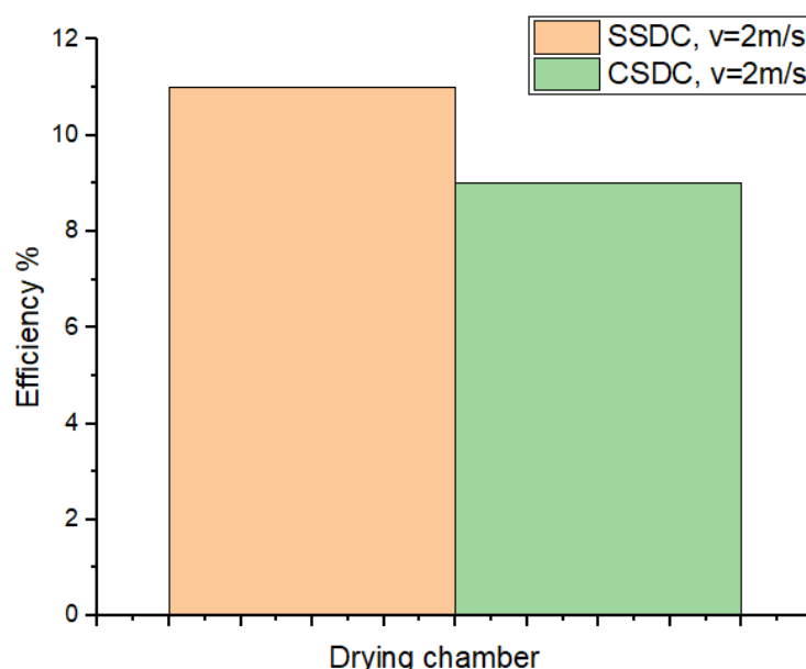
Fig. 13. Drying chamber efficiency of the SSDC and CSDC
