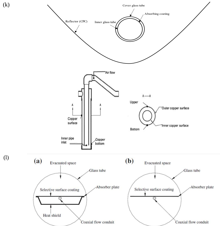
Fig. 2 Various designs of ETSACs: (a) shapes of absorber tubes by Kim and Seo [53]; (b) schematic of the U-type evacuated tube solar collector by Naik et al. [56] for (i) cross-section and (ii) illustration; (c) schematic diagram of H-type & T-type models by Ataee and Ameri [57]; (d) schematic view of the solar evacuated tube collector [58]; (e) Working principles of the (i) evacuated tube-integrated collector storage solar heater and (ii) flat micro-HP arrays by Wang et al. [60]; (f) schematic of the all-glass ETSACs by Liang [63]; (g) schematic diagram of the evacuated tube solar heaters by Abu Hamed and Alkharabsheh [64]; (h) arrangements for the flow of air in the experimental setup by Kumar et al. [66]; (i) schematic designs for the head of evacuated tubes by Yadav and Bajpai [67]; (j) EGATC construction by Zakaria et al. [68]; (k) additional reflector for a U-shaped copper tube heat exchanger by Wang et al. [71]; and (l) cross-sections of evacuated tubes (a) with and (b) without a heat shield by Zhang et al. [72].
