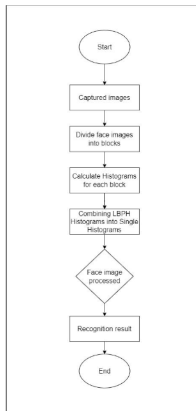
Fig. 1. Flowchart for LBPH Model
