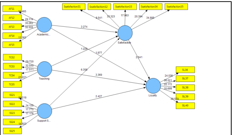
FIGURE 3 Bootstrapping Assessment
