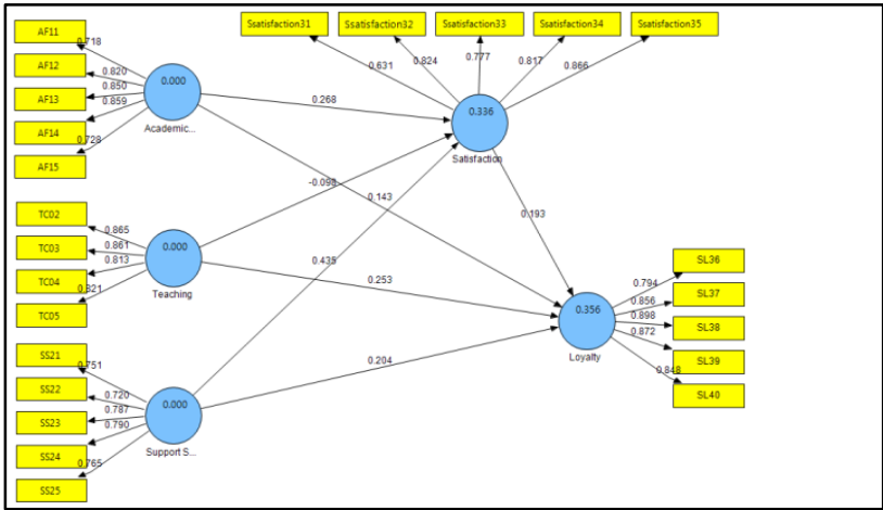
FIGURE 3 Bootstrapping Assessment
