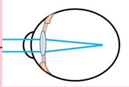
Myopic eye
