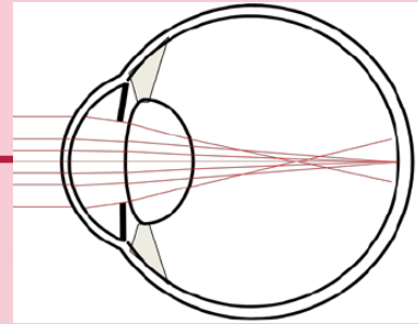
Aberrated eye
