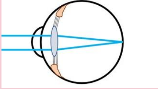
Normal eye
