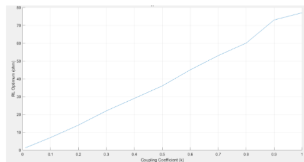
Figure 5: the graph of optimum load impedance against the coupling coefficient
