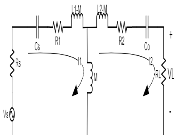
Figure 1: The series-to-series T-equivalent circuit
