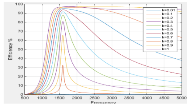
Figure 4: The graph of power transfer efficiency at load impedance of 100\Omega
