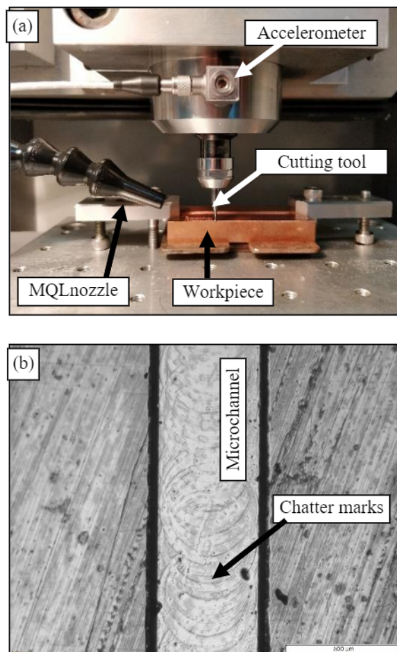
Figure 1. (a) Experimental setup of MQL micromilling and, (b) optical image machined microchannel with chatter marks.
