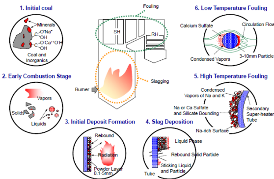
Figure 1: Slagging and Fouling Deposit Formation (modified from Couch,2006) [5]
