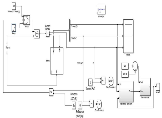
Fig.1. Overall dynamic charging model of MATLAB Li-ion battery
