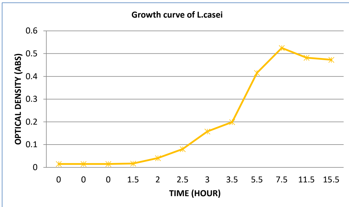
Figure 3. Growth curve of L. casei within 24 hours period
