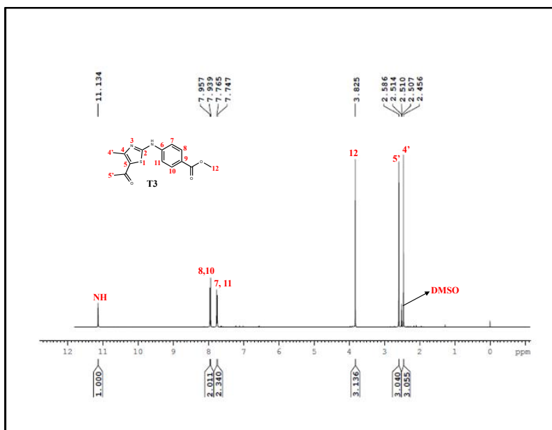
Figure 3. ^1\text{H} NMR spectrum of 5-acetyl-4-methyl-2-(methyl-4-aminobenzoate)-1,3-thiazole ( T3 )
