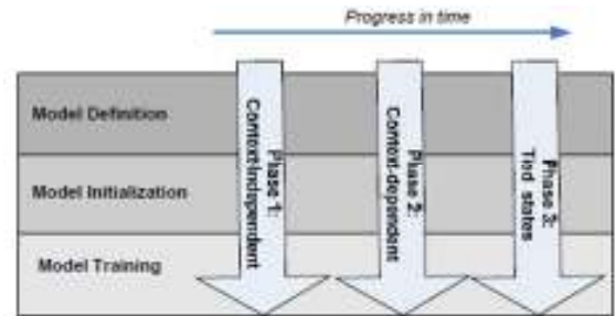
Figure 4. Acoustic model training phases for Sphinx 3 [4].
