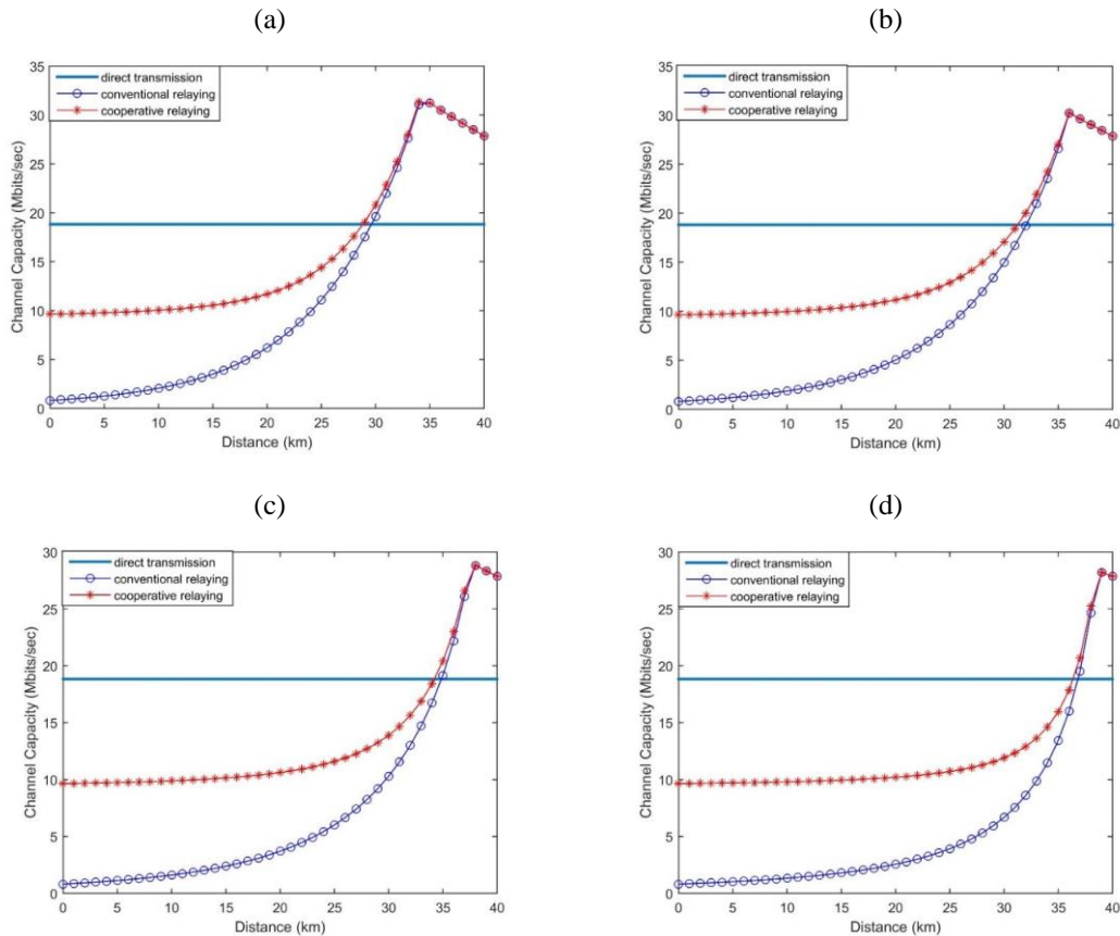
Figure 4 Channel Capacity for non-linear 3-node AWGN relay channel (a) b = 5 , (b) b = 10 , (c) b = 15 , (d) b = 20
