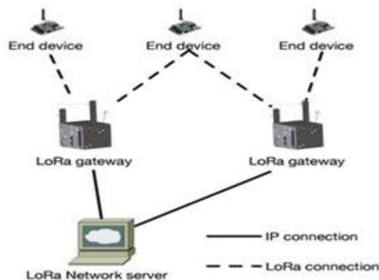
Figure 2. The architecture of LoRa which include three dissimilar devices [6]
