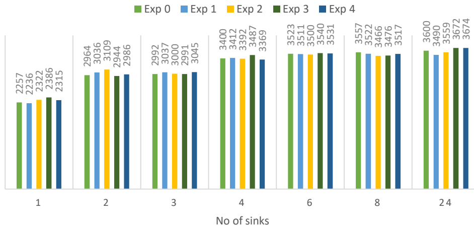
Figure 13. Number of lost packets due to shadowing
