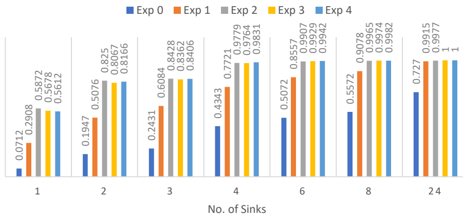
Figure 14. Channel Throughput Degradation without the effect of Shadowing
