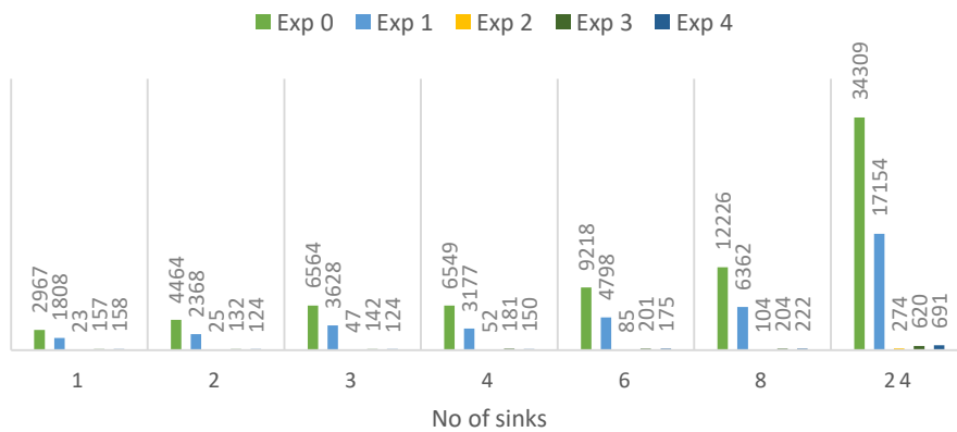
Figure 17. Number of collided packets because of Shadowing
