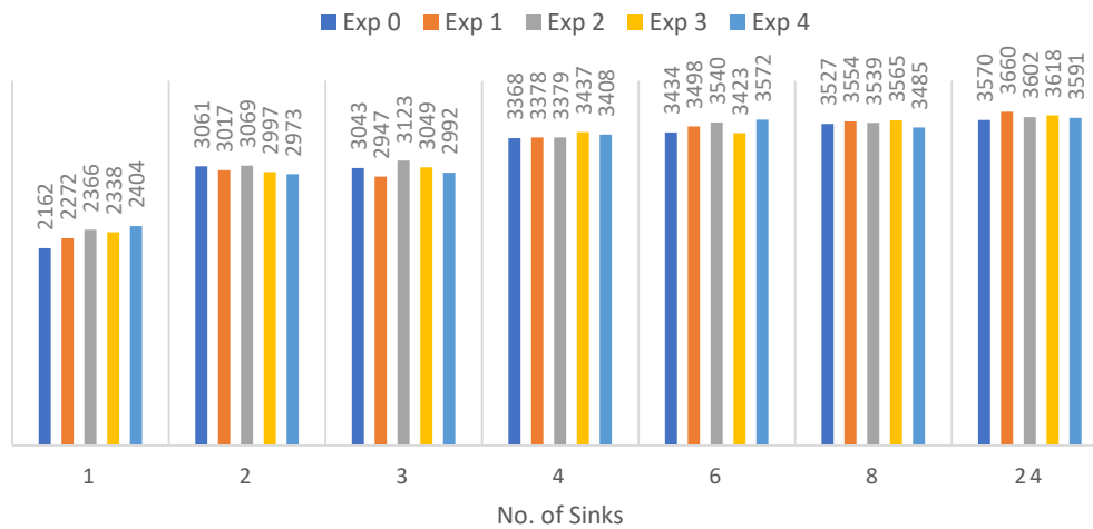
Figure 12. Number of lost packets without shadowing
