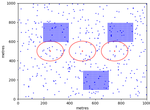
Figure 5. The number of sink is 3, and the number of nodes are 1600
