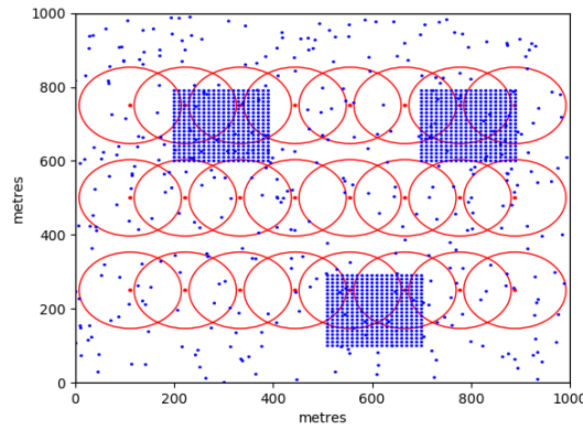
Figure 9. The number of sink is 24, and the number of nodes are 1600
