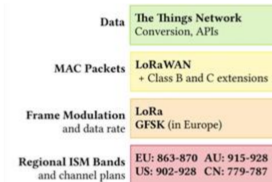
Figure 1. LoRaWAN stack [4]
