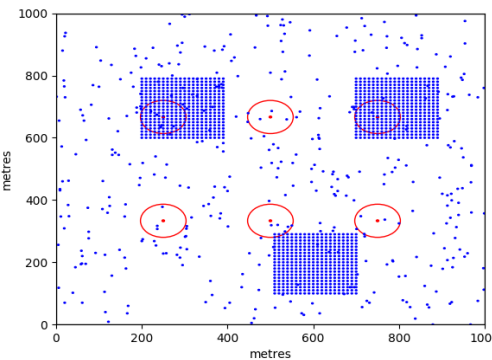
Figure 7. The number of sink is 6, and the number of nodes are 1600
