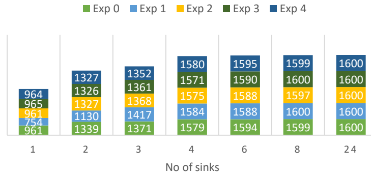
Figure 11. Number of Connected Nodes with Shadowing Effect
