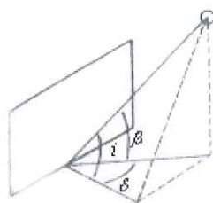
Figure A.3. Superimposed shadow angle protractor on sun path diagram
