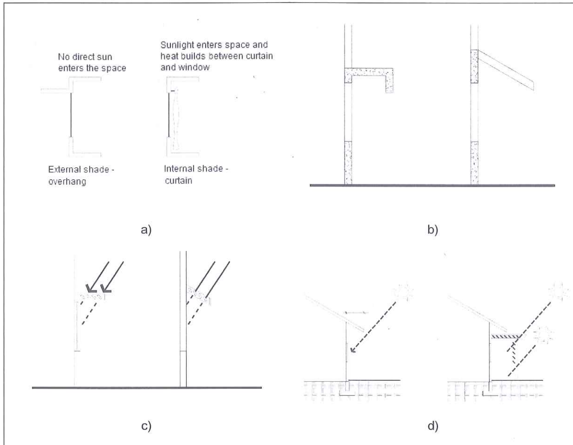
Figure 6. Sun shading devices
