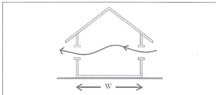
Figure 12. Cross ventilation
