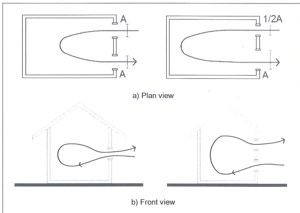
Figure 10. Single sided ventilation
