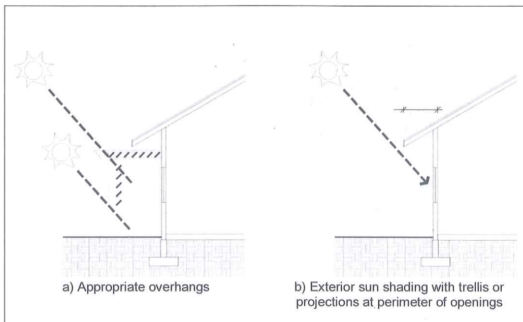
Figure C.1. Control of solar penetration
