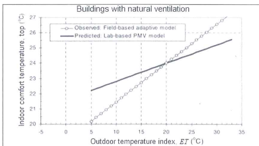
Figure 15. Divergence of actual comfort sensation observed in the field compared to PMV model prediction found in naturally ventilated spaces
