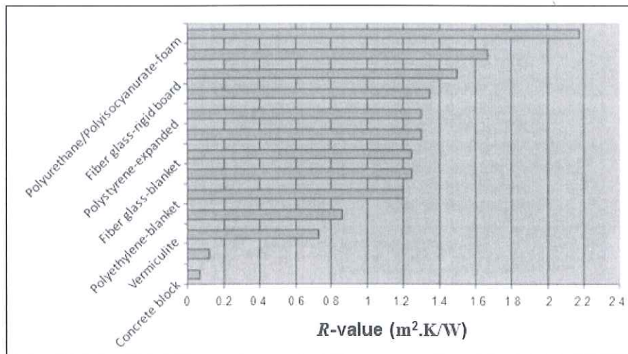
Figure C.6. R-value of common building materials based on 50 mm thickness
