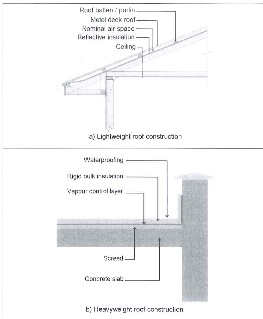
Figure 5. Roof assembly
