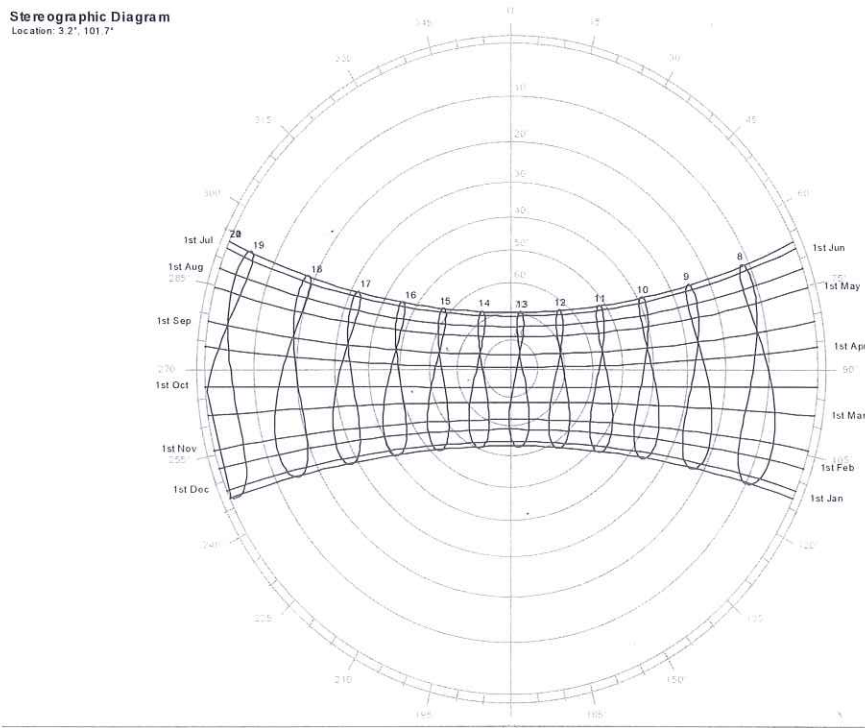
Figure A.2. Sun path diagram
