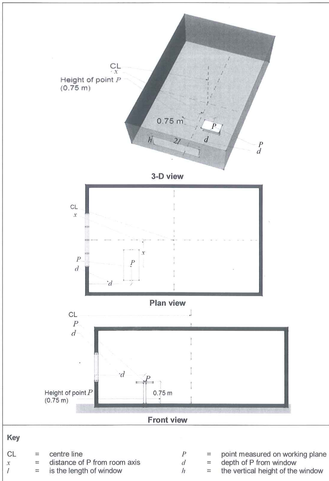
Figure 3. Room geometry
