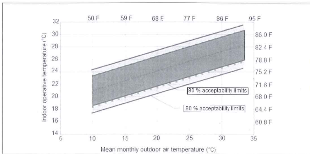
Figure 16. ANSI/ASHRAE Standard 55 adaptive thermal comfort chart
