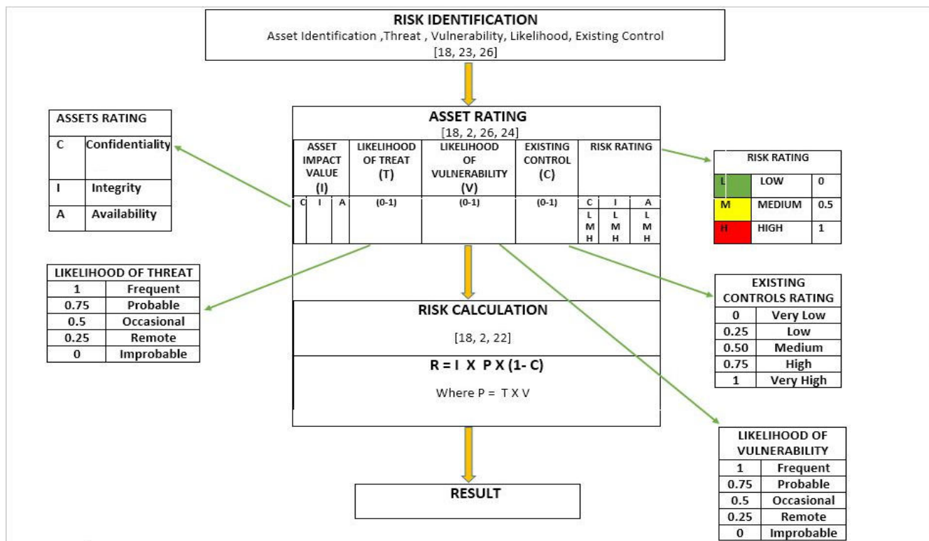
Figure-3. C-RAM Model Adapted from [2, 18, 22, 23, 24, 26].
