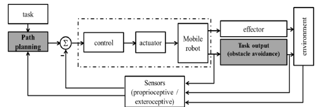
Figure 4. Block diagram of the mobile robot hardware
