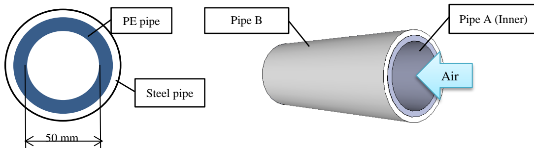
Figure 3: A cross section of two pipes in a hybrid pipe system
