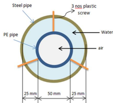
Figure 4: A cross-section of the insulated hybrid materials.
