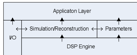
Fig. 4: Layered architecture of the developed software tool,
