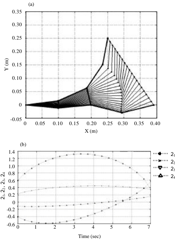
Fig. 7(a-b): 4-link robot for a point close to the boundary(a) IK configuration and (b) Joint values
