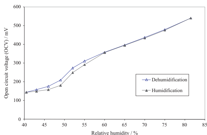
Fig. 4. OCV response of Zn/MCM-41/air cell as a function of relative humidity.
