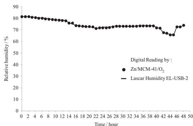
Fig. 6. Relative humidity measurement utilizing a digital humidity sensor and OCV readings from the Zn/MCM-41/air cell.
