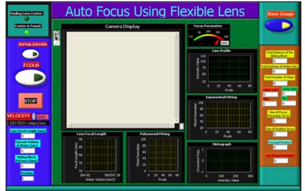
Fig. 5: User interface for the flexible lens system.
