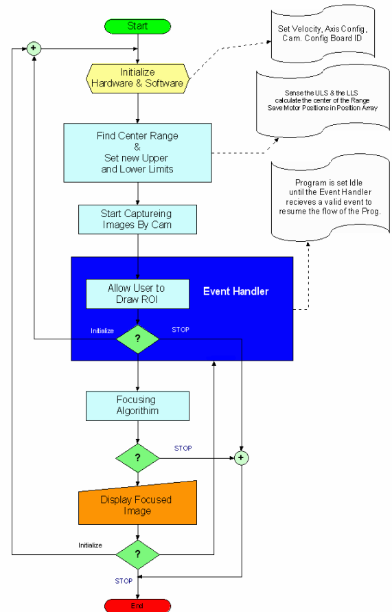
Fig. 6: Flow-chart of autofocus process
