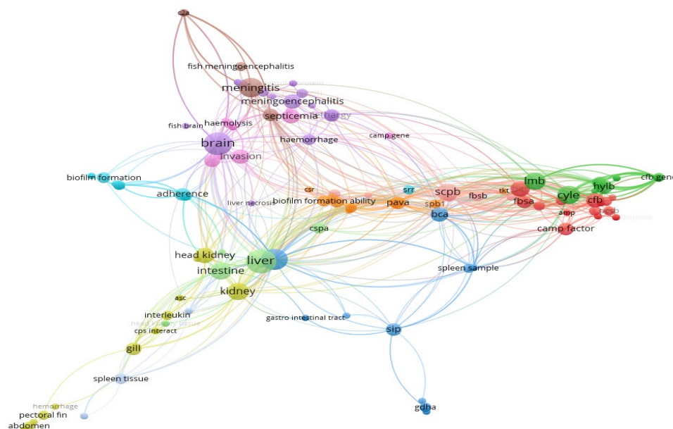
Figure 1 Relation between all keywords (Virulence genes, organs, clinical signs)
