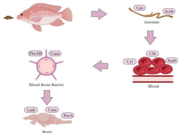
Figure 5 Streptococcus agalactiae infection pathway through the intestine
