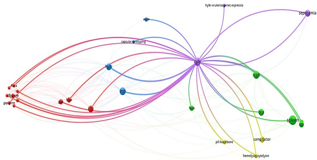
Figure 3 Relation between CylE with virulence genes, organs and clinical signs
