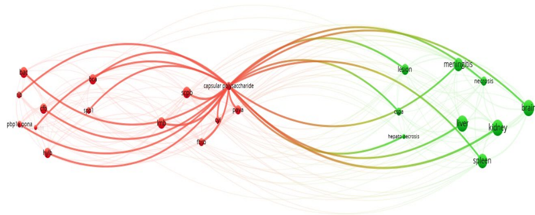
Figure 2 Relation between capsular polysaccharide with virulence gene, organs and signs
