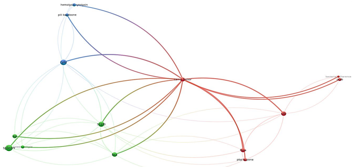
Figure 4 Relation between CAMP-factor with virulence genes and organs
