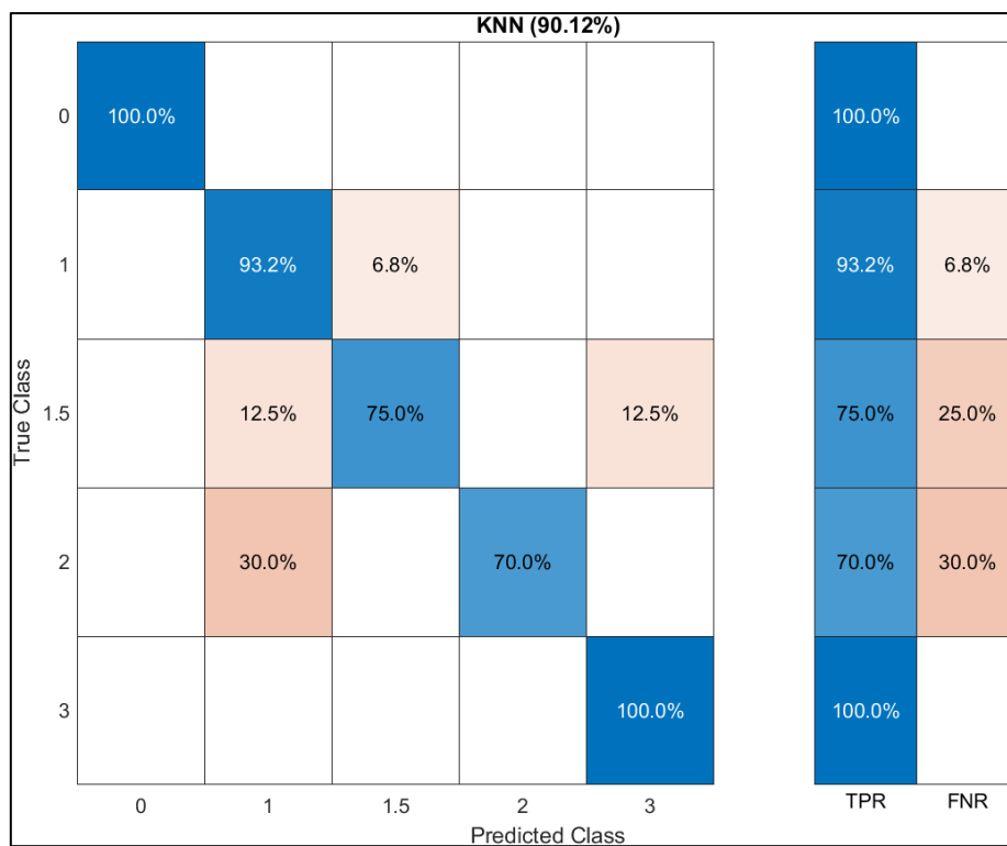
Figure 4: Confusion Matrix and Performance Metrics of KNN Model for Flexion Movement
