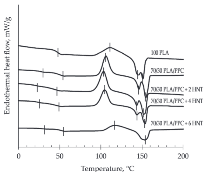
Fig. 6. DSC thermograms of PLA/PPC/HNT nanocomposites
