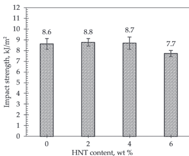
Fig. 5. Impact strength of PLA/PPC 70/30 with different HNT content
