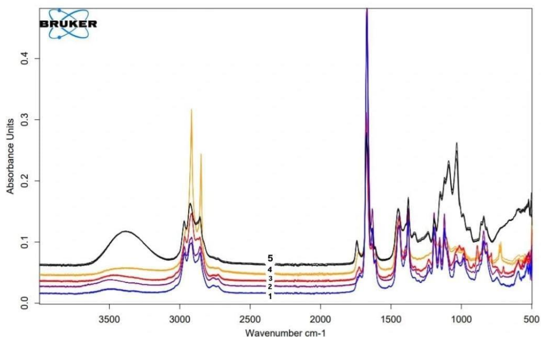
Figure 4. FTIR spectra of distilled lemongrass (1), Soxhlet extracted lemongrass (4) and market samples A (2), B (3) and C (5).
