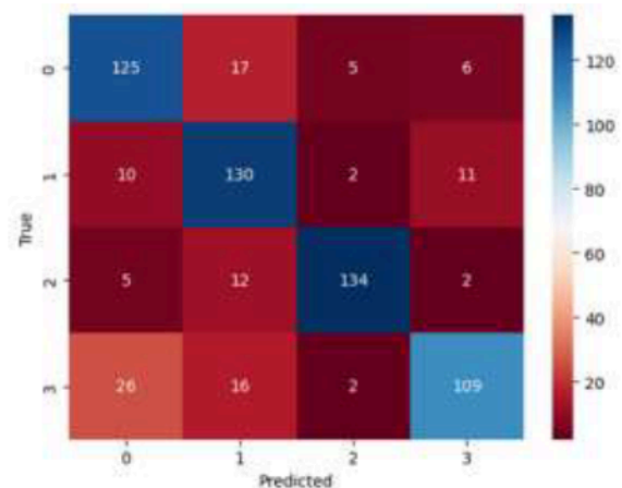
Fig. 18 The Confusion Matrix of ViTs
