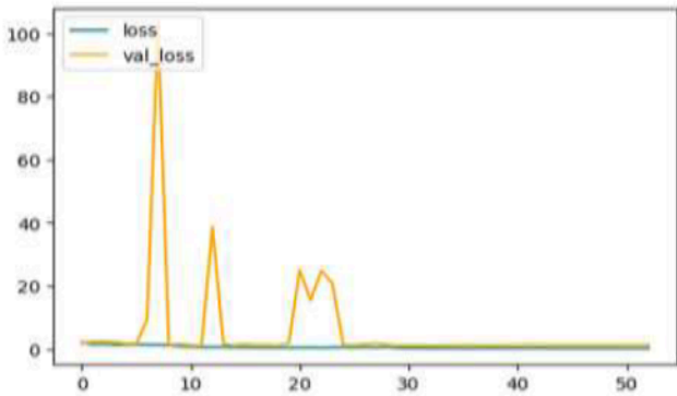
Fig. 11 The Loss Rate of ResNet-50 from 0-53 Epochs.
