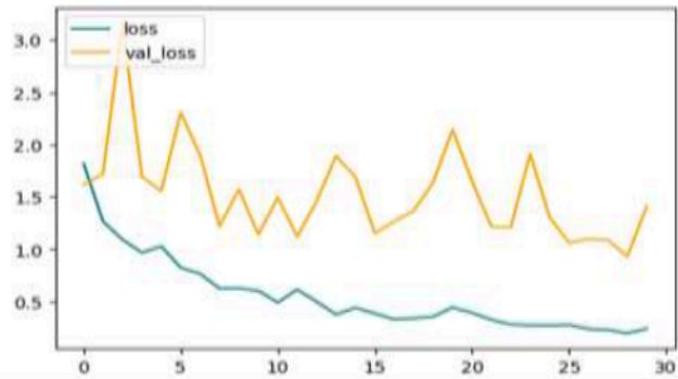
Fig 12 The Loss Rate of ResNet-50 from 0-33 epochs.
