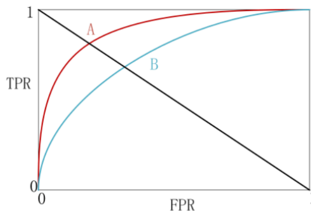
Figure 8. TPR FPR curve for two classifiers [29]
