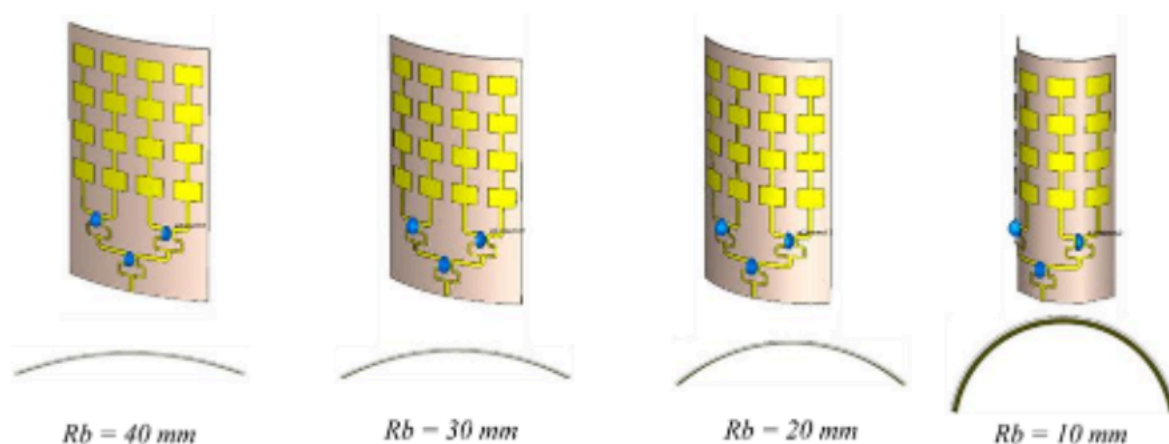
Figure 4. Bending configurations of the antenna with radius of curvatures of 40 mm, 30 mm, 20 mm and 10 mm
