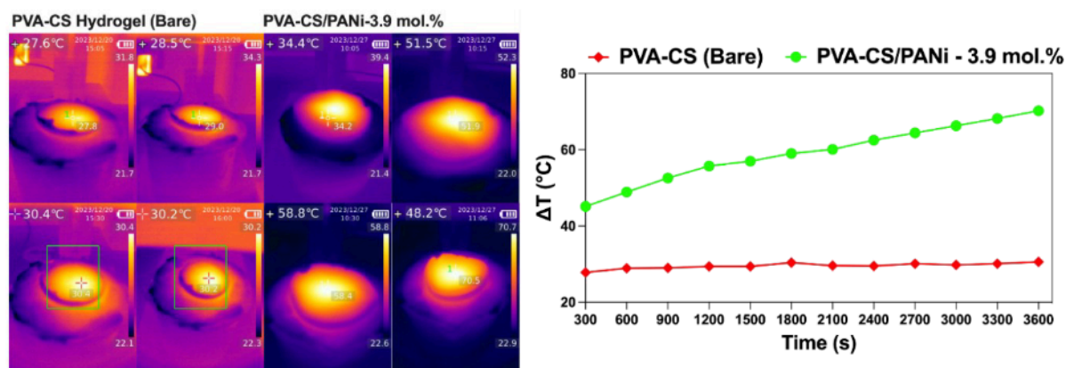
Figure 10. Water heating ( \Delta T - the temperature difference between the temperature before and after irradiation) was recorded in different illuminations over 1 hour period.
