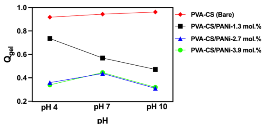
Figure 7. Equilibrium of PVA-CS/PANi with different concentrations of PVA and PVA-CS hydrogel corresponding to pH
