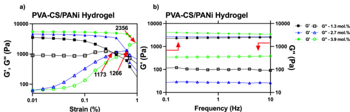
Figure 5. Rheology studies for PVA-CS/PANi with different concentrations of PVA (a) Strain amplitude of 1.3 mol.%, 2.7 mol.% and 3.9 mol.%; (b) Frequency-sweep of 1.3 mol.%, 2.7 mol.% and 3.9 mol.%
