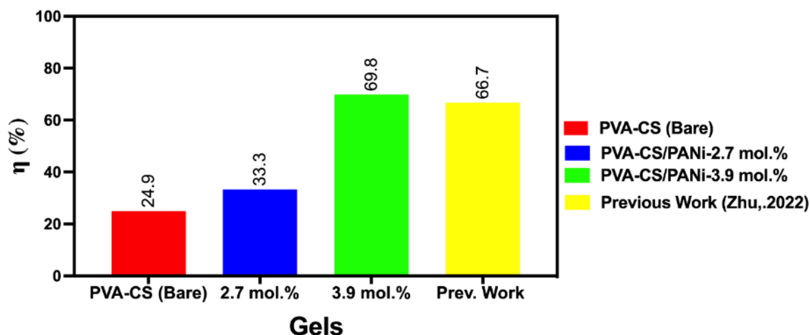
Figure 9. SVG efficiency of PVA-CS hydrogel and PVA-CS/PANi hydrogel
