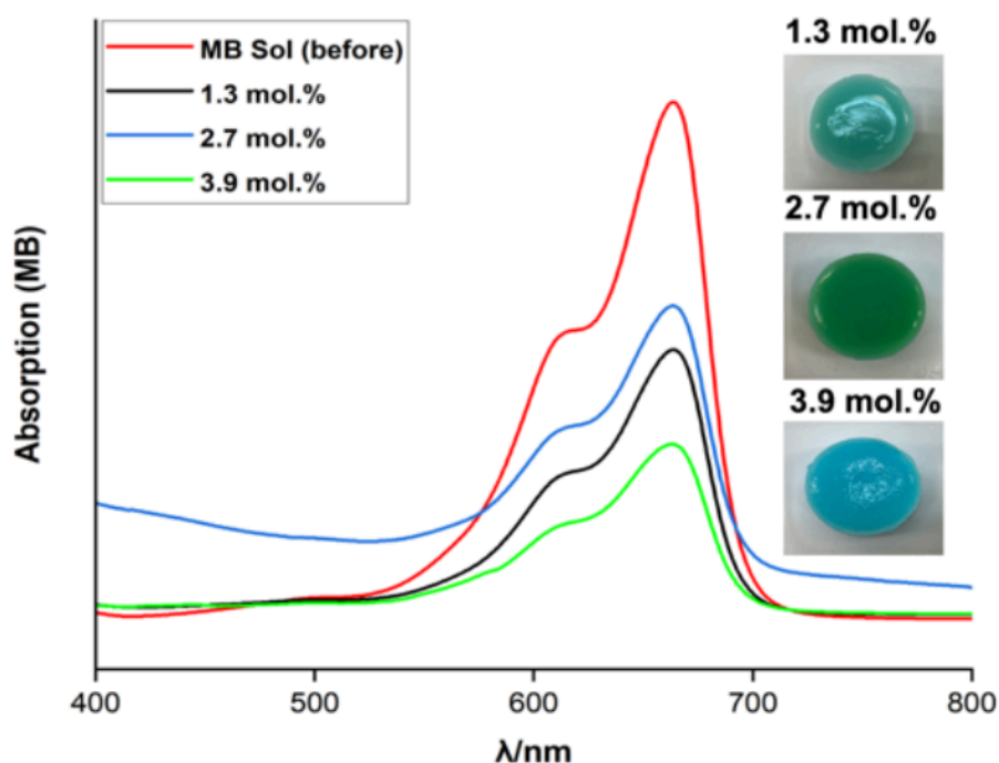
Figure 8. PVA-CS hydrogel UV-vis absorption of Methylene Blue (MB)
