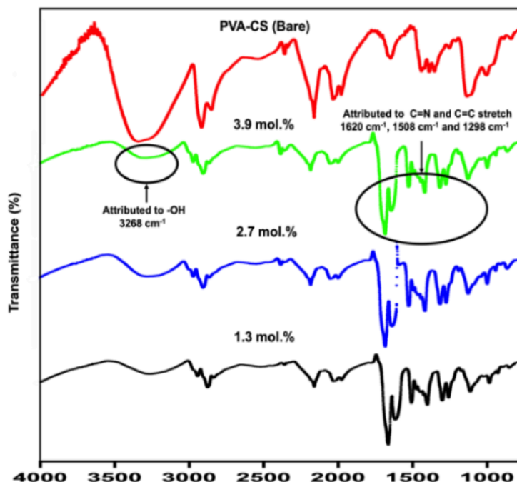
Figure 3. FTIR spectra of the chemical compositions of PVA-CS hydrogel and PVA-CS/PANi hydrogel
