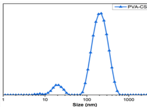
Figure 1. Particle size distribution of PVA-CS particles obtained from DLS analysis.
