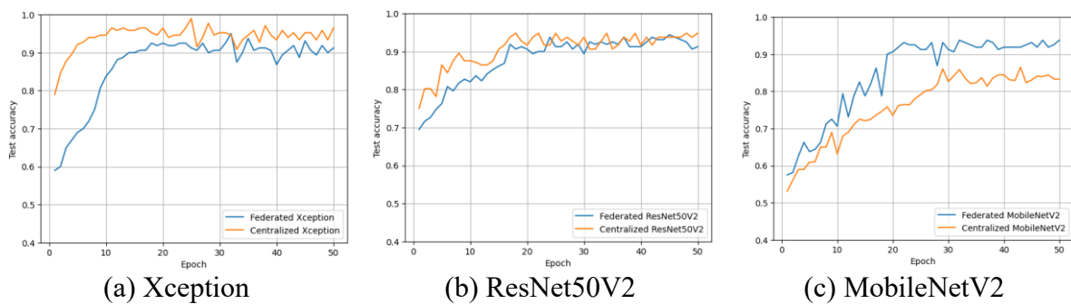
Figure 4. Comparison of the centralized and Federated learning
