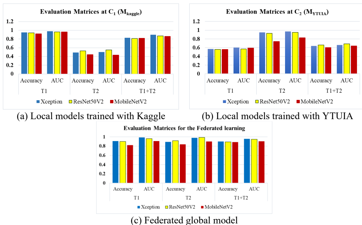
Figure 5. Evaluation matrices after testing with different test sets
