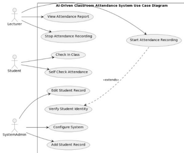
Fig.5.Use Case Diagram
