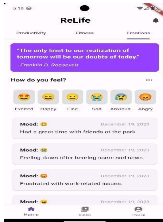
Fig. 5. Emotions Page
