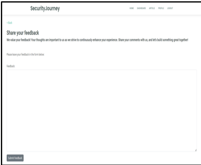
Fig. 15 Feedback Page
