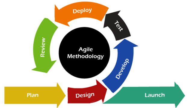
Fig. 1 Agile Methodology
