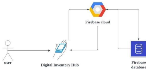
Fig. 4 System Architecture
