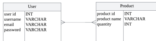
Fig. 8 Database Design
