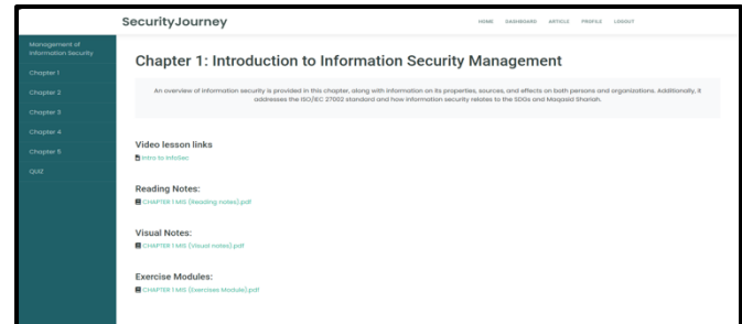
Fig. 12 Chapter Page
