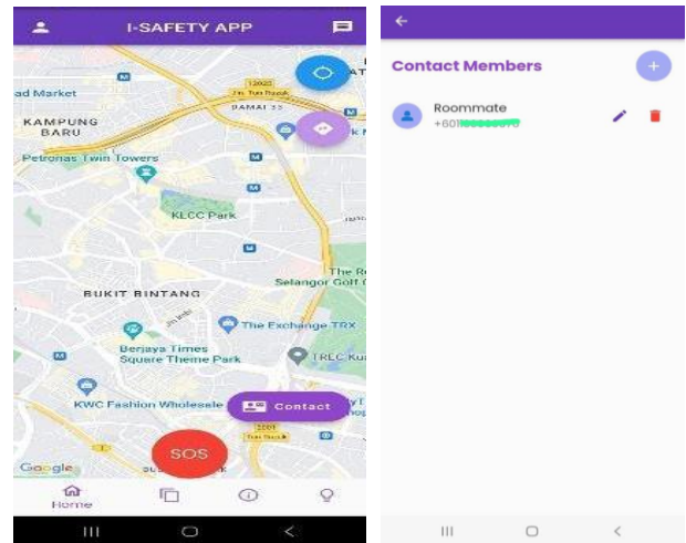
Fig. 6. Home Screen.
