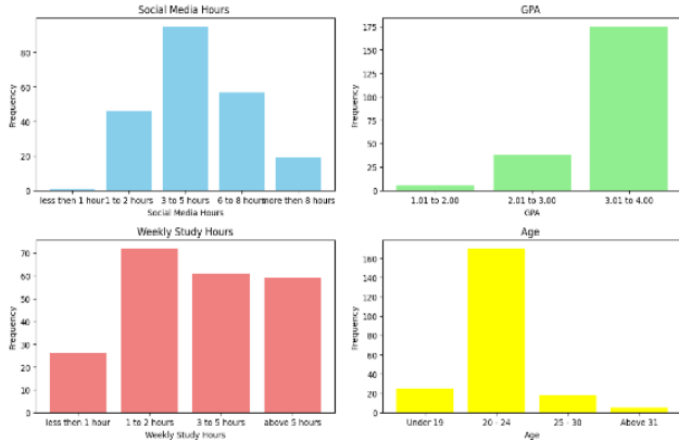
Fig. 2. Histogram Distribution
