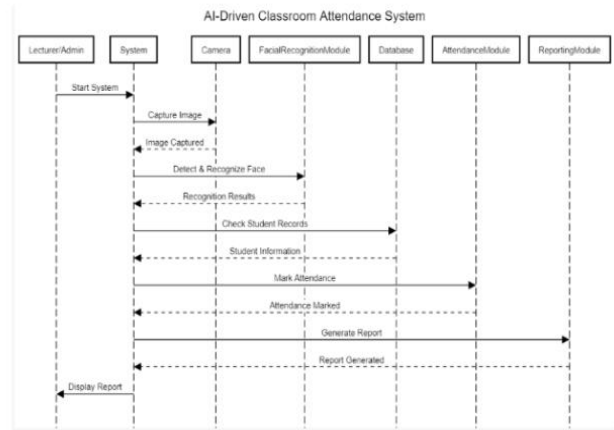
Fig. 6. Sequence Diagram
