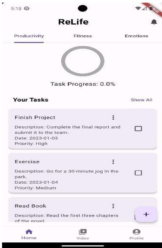
Fig. 3. Productivity Page
