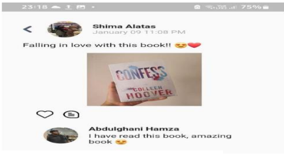
Fig.20. Comment Interface
