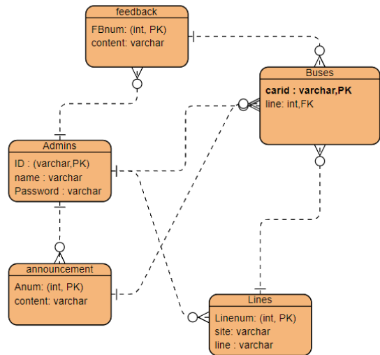
Fig. 4. Database design
