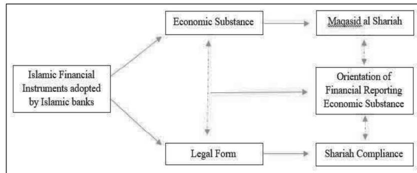
FIGURE 6: CONCEPTUAL FRAMEWORK
