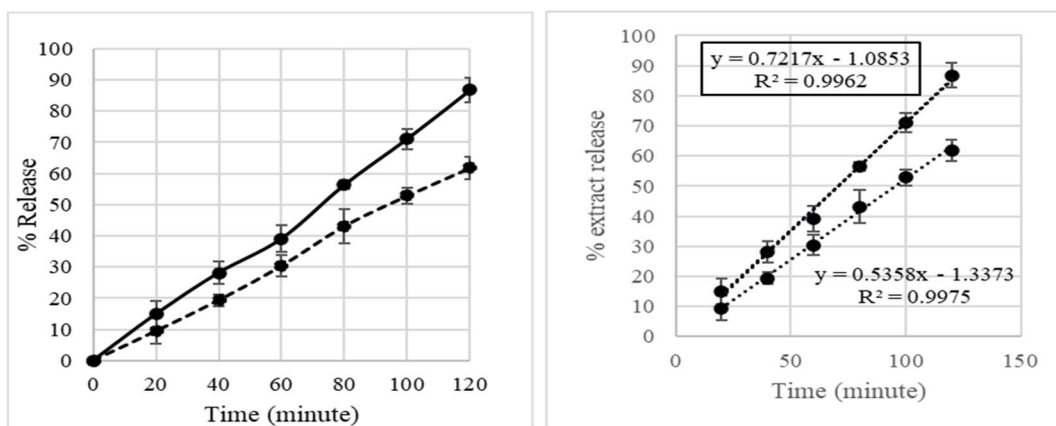
Figure 2. Release profile of capsules F1 and F2
