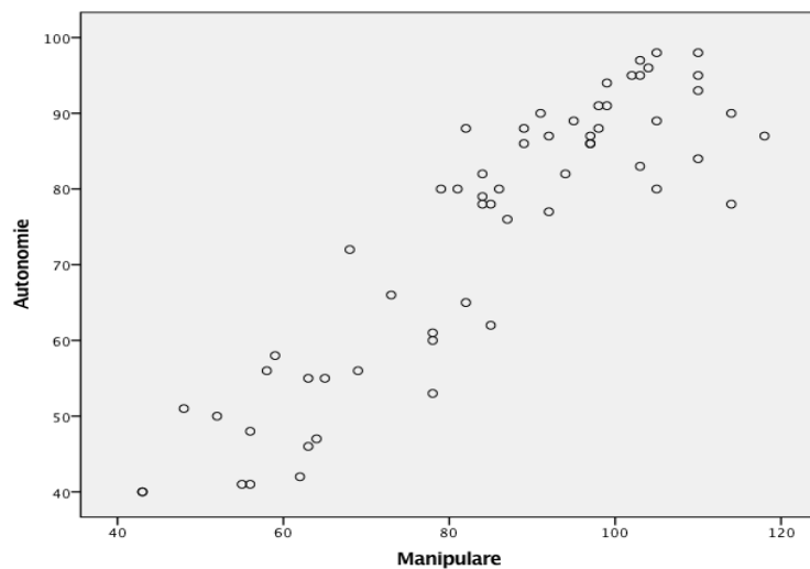
Fig. 4.12 Manipulation – autonomy
