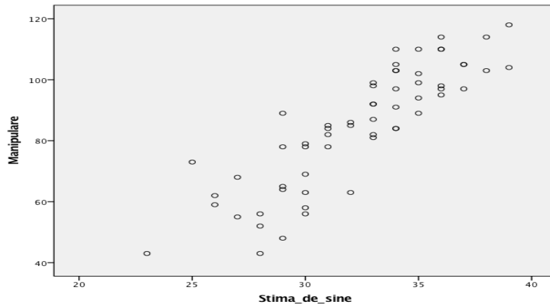
Fig. 4.3 Manipulation – self-esteem
