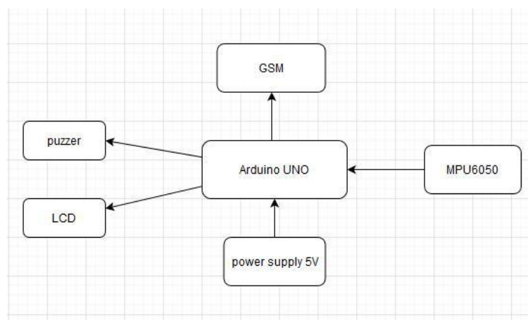
Figure 1 : Block Diagram of Smart Assistant for Paralyzed Patient
