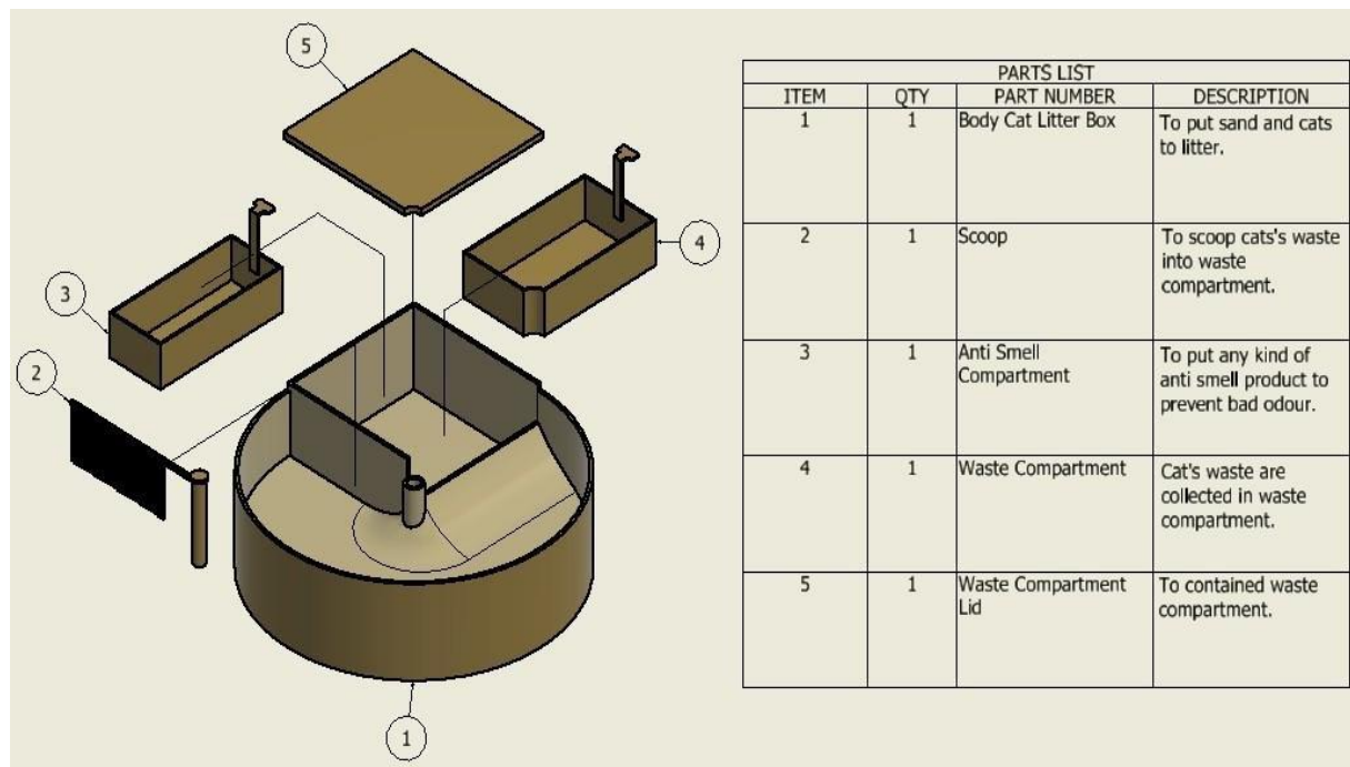
Figure 2: Final design
