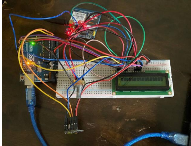
Figure 2 : Circuit diagram project Smart Assistant for Paralyzed Patient
