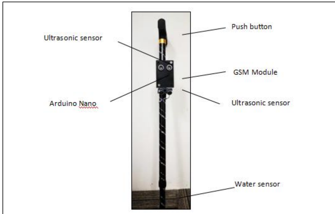
Figure 3: The Finished Prototype
