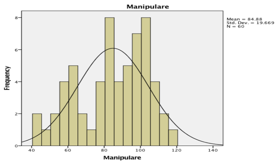
Fig. 4.4 Manipulation
