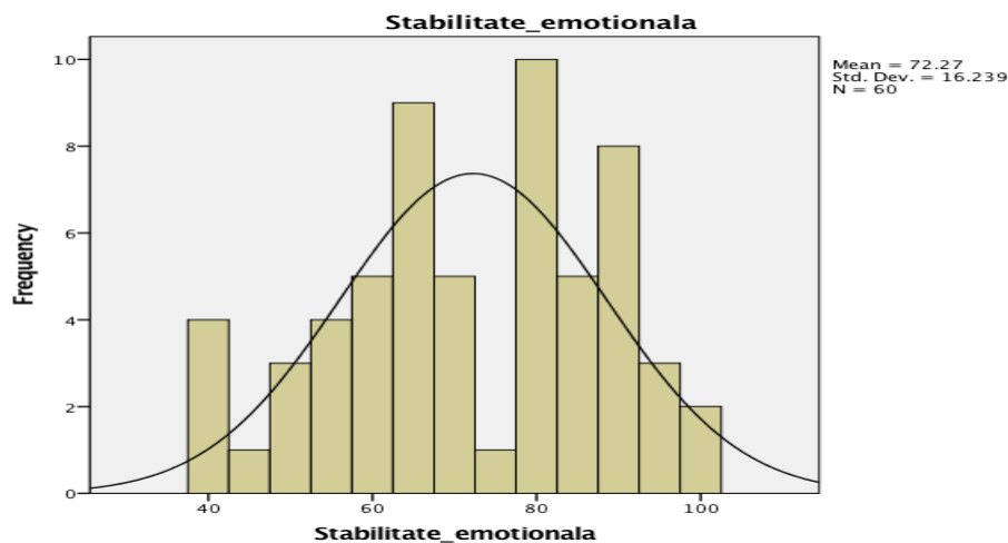
Fig. 4.8 Emotional stability
