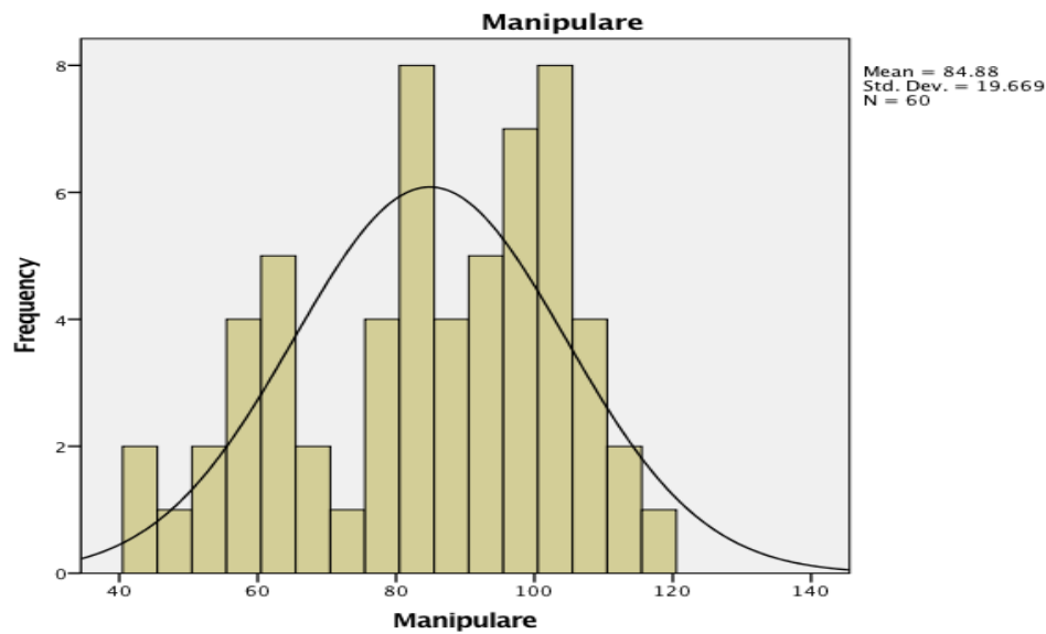
Fig. 4.7 Manipulation
