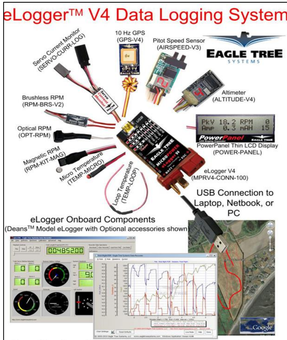
Figure 2: eLogger System
