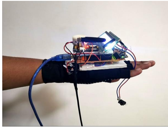
Figure 4 : Practical circuit project Smart Assistant for Paralyzed Patient
