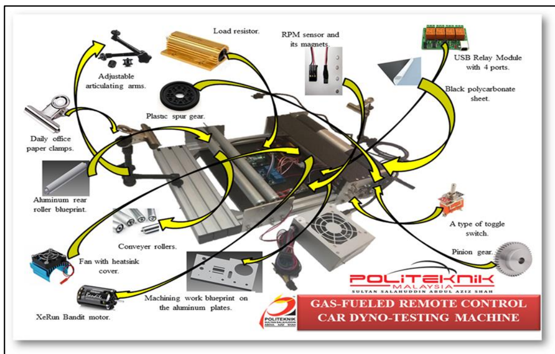
Figure 1: Training Kit
