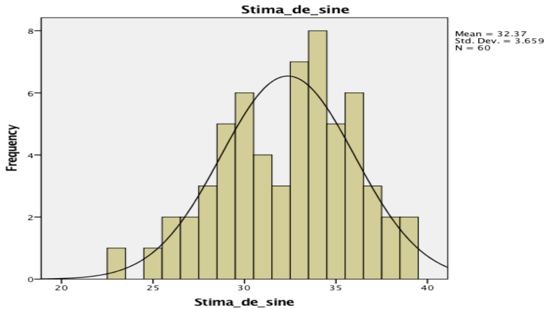
Fig. 4.2 Self-esteem
