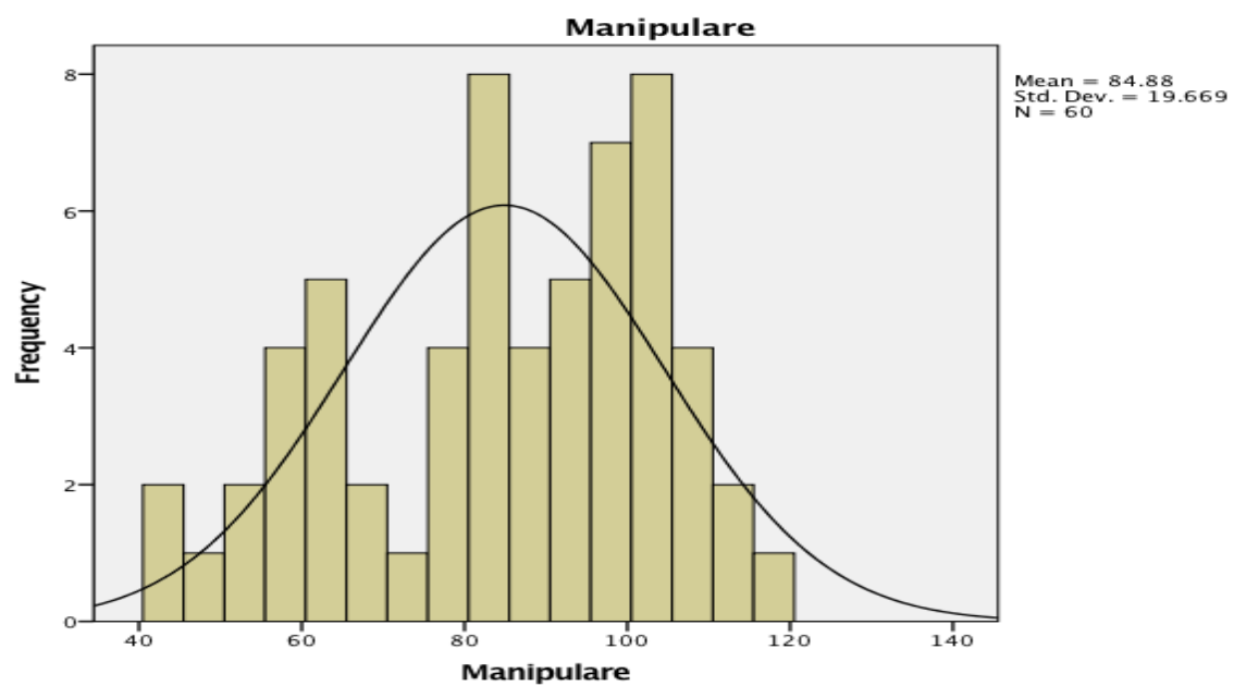
Fig. 4.1 Manipulation
