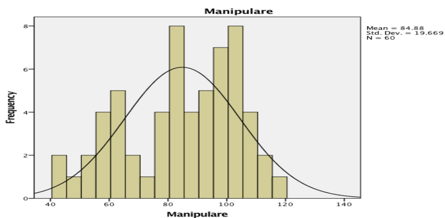
Fig. 4.10 Manipulation
