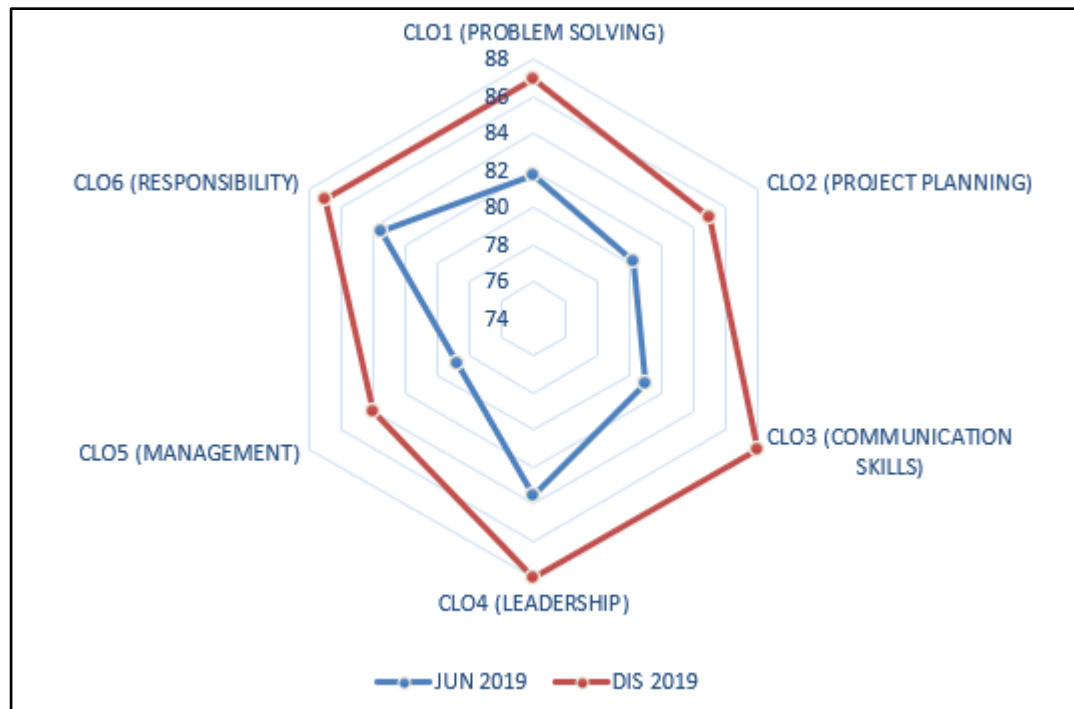
Chart 4: CLOs Performance
