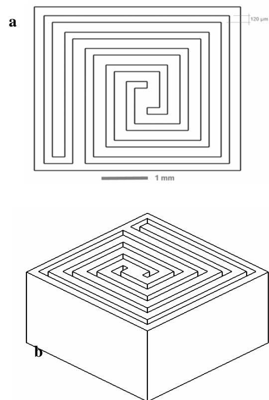
Figure 4. Design of micro swiss-roll combustor mold cavity of 120 \mu\text{m} channel width (a) top view, and (b) isometric view (Ahn and Ronney, 2005).
